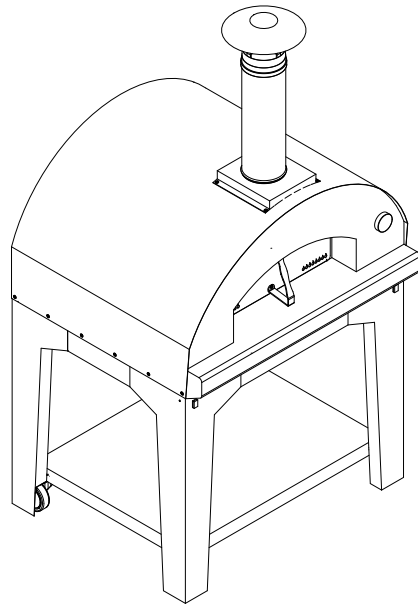
ISOMETRIC VIEW
